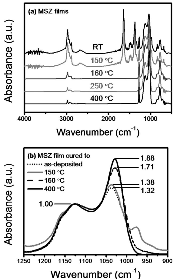
Figure 5. Transmission FT-IR spectra of the MSZ films cured at various temperatures: (a) 500–4000 \text{cm}^{-1} and (b) 900–1250 \text{cm}^{-1} .
